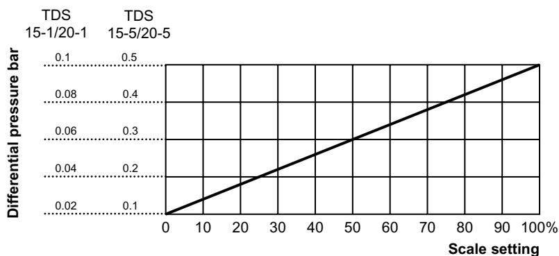
Relation between Scale Setting and Differential Pressure
